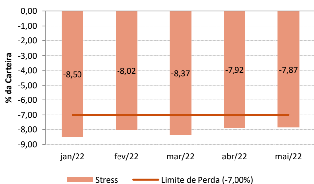
Stress Test
